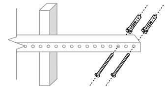
E-Z Toggles at 2" & 5" from rail end
